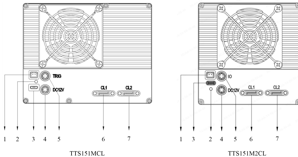
Fig.6 Interfaces of Camera
