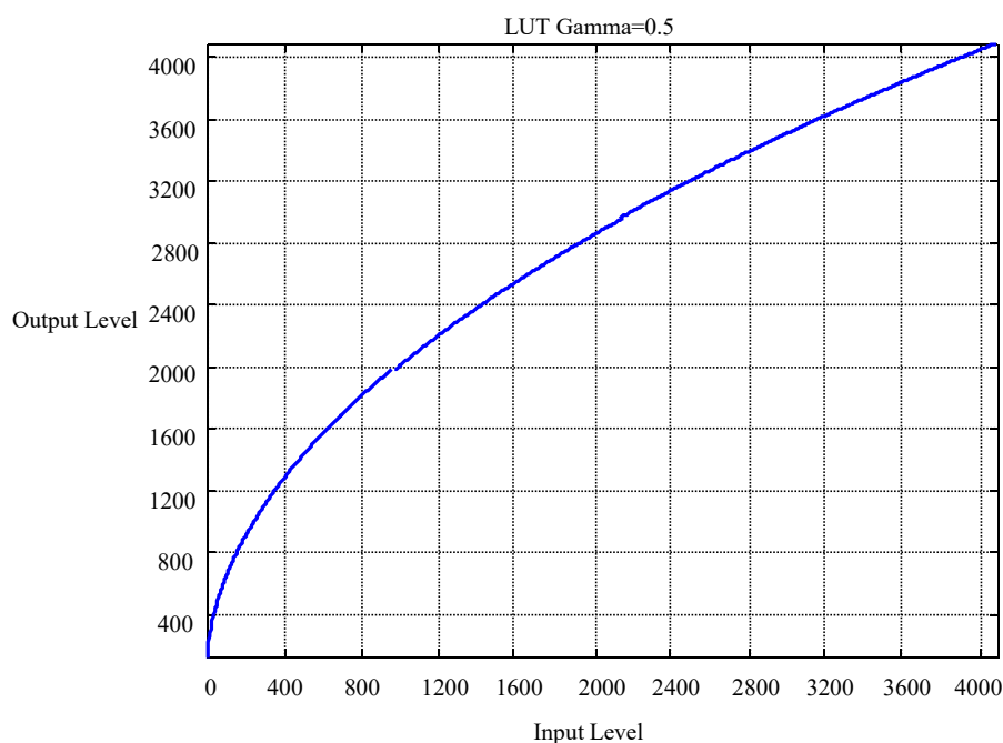
Fig.19 LUT Gamma = 0.5
