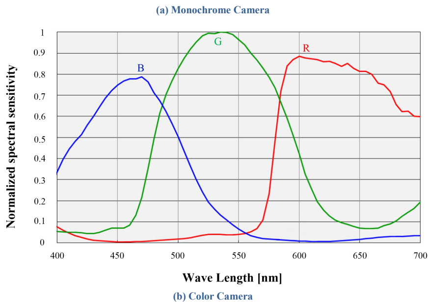
Fig.3 Spectral Response of Camera
