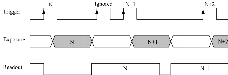
Fig. 14 External Trigger Interval is Too Short
