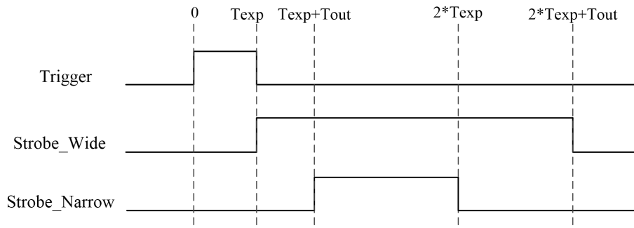
Fig. 25 Exposure Time is greater than Readout Time
