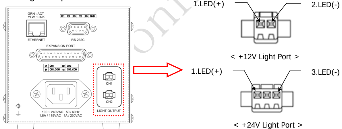
< +12V Light-Output Pin-List >
