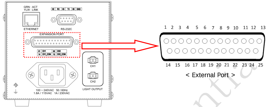
< External Input Port Pin-List >
