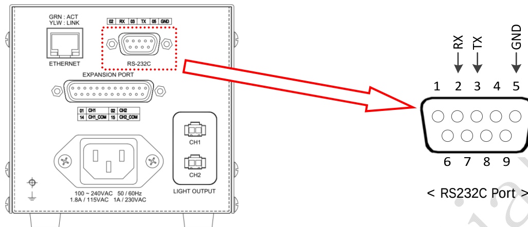
< RS232C Pin-List >
