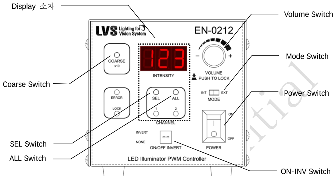
< EN-02 Series 전면부 >
