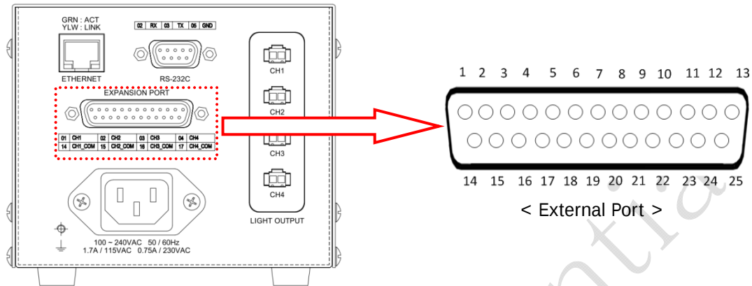
< External Input Port Pin-List >
