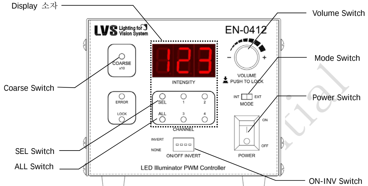
< EN-04 Series 전면부 >
