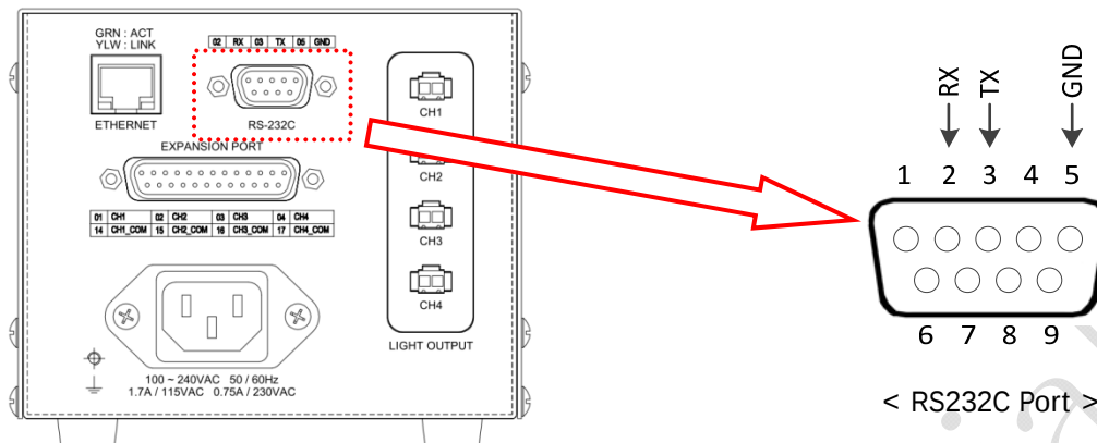
< RS232C Pin-List >
