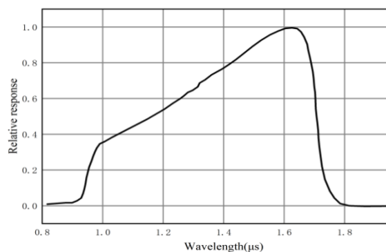
Spectral response
