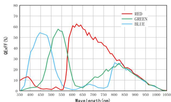
Spectral response
