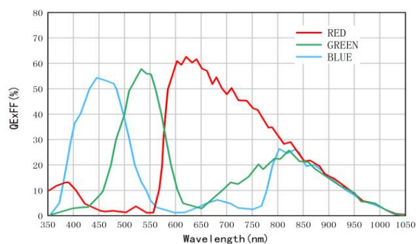
Spectral response
