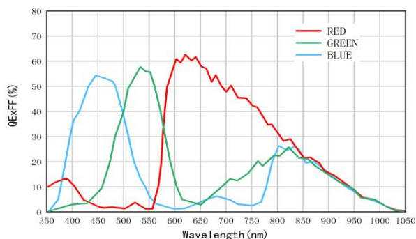
Spectral response
