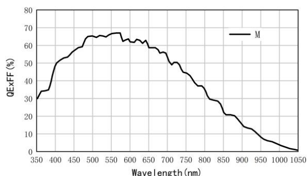
Spectral response
